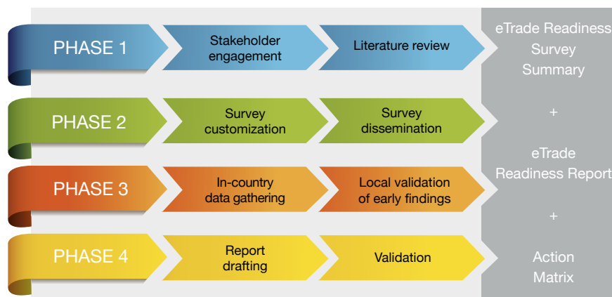
Figure 2: Assessment methodology
